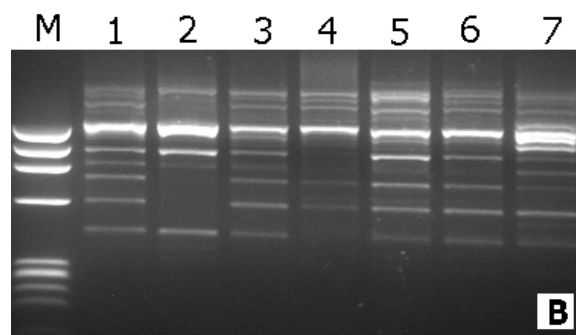
Figure 8: RAPD profile for the (7) Sweet Sorghum (Ankolib) accessions as detected by primer B (OP-B12). Lanes (1) to (7) represent the (7) accessions M: Φ X174 RF Hae III marker.
