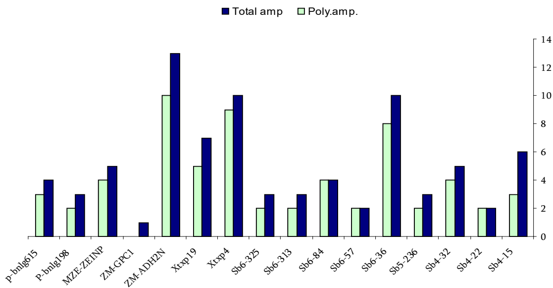
Figure 11: SSR histogram showing the levels of polymorphism as revealed by each SSR primer pairs.
