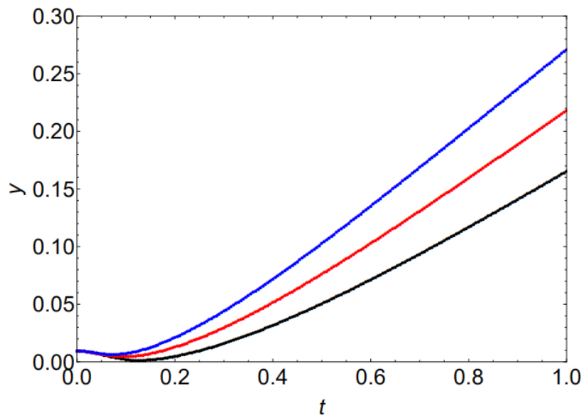
Figure 1: The temperature dependence of the inverse of the reduced magnetic susceptibility y when \alpha = 0.98 , \beta = 10^{-4} , \chi_0 = 1000[1/K] , y_0=0.01 , y_1=1, y_2=30 (the black line), 50(the red line), 80(the blue line), respectively.
