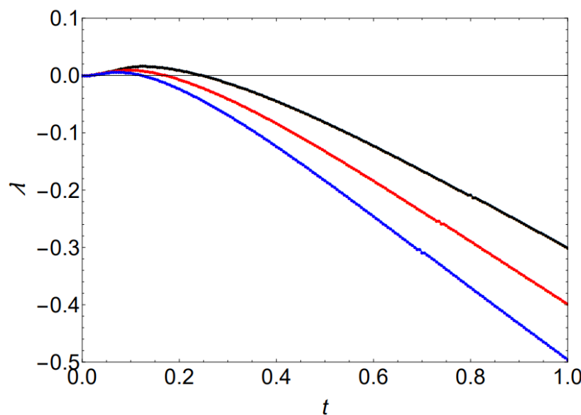
Figure 2: The temperature dependence of the \lambda when \alpha = 0.98 , \beta = 10^{-4} , \chi_0 = 1000[1/K] , y_0=0.01 , y_1=1, y_2=30 (the black line), 50(the red line), 80(the blue line), respectively.
