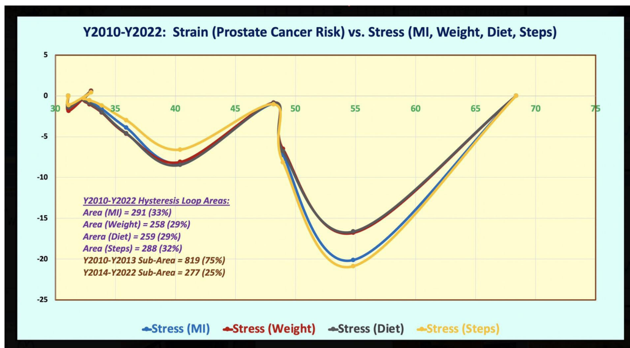
Figure 4: Stress-strain diagram of prostate cancer risk % with 4 hysteresis loops via VGT analysis in a space-domain.
