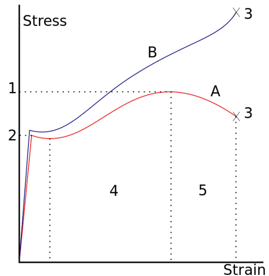
A stress-strain curve typical of structural steel.
